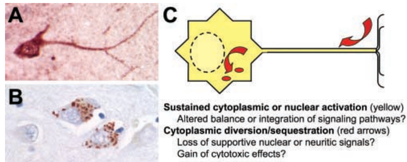
Fig. 2. Distinct subcellular localization patterns for phosphorylated ERK1/2: Mechanistic implications. Neurons exhibiting ERK1/2 activation typically display several general immunohistochemical patterns including diffuse labeling restricted to processes or soma and diffuse nuclear and cytoplasmic staining, as observed in this ischemic human neuron (A). Degenerating populations of neurons may also display discrete, cytoplasmic labeling for phospho-ERK1/2, as illustrated by these hippocampal neurons from a patient with dementia (B). Hypothetical effects related to differences in subcellular localization of activated ERK1/2 are schematically illustrated (C). Although compartmentalization of activated ERK1/2 does not necessarily imply that downstream signaling effects are limited to these compartments, it is probable that different subsets of scaffolding anchors, target proteins and regulatory phosphatases are involved. Cellular integration of divergent downstream effects will determine the favorable vs. detrimental outcomes to neuronal injury involving ERK1/2 signaling pathways. In addition, the potential contribution of ERK1/2 activation in non-neuronal CNS cell types must be considered at the organism or tissue level.
